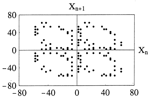
Figure 4. An orbit of (18) for \sigma = 3 , H = 10 , X_0 = 11 , X_1 = 17 . Period is 132.
